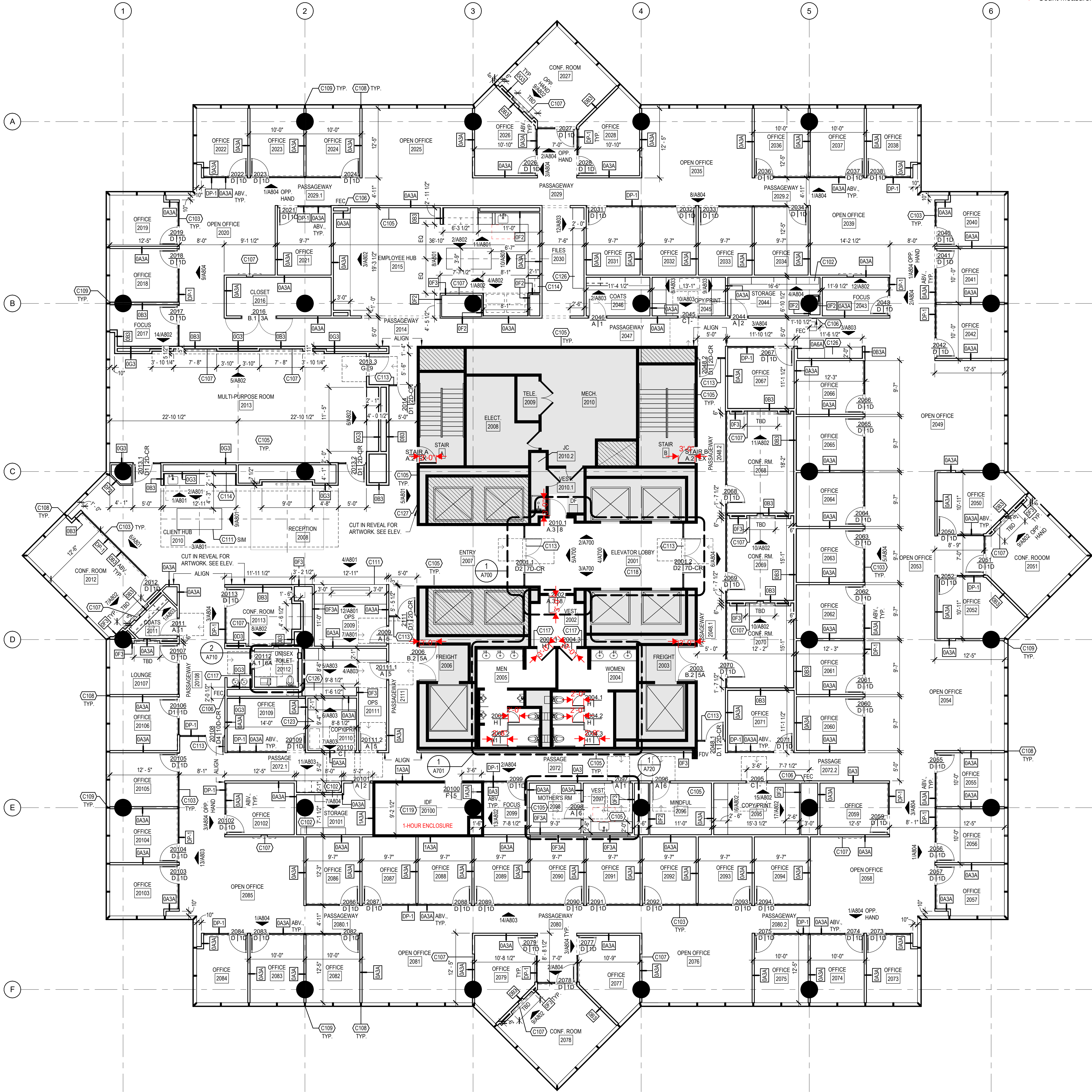
1 FLOOR PLAN - LEVEL 20 1/8" = 1'-0"
